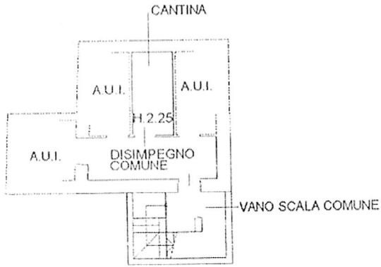
PIANO INTERRATO
