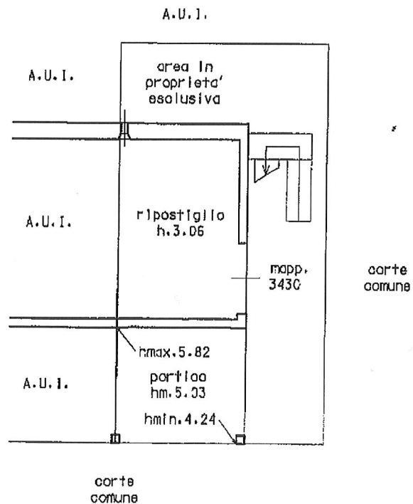
PIANO TERRA
